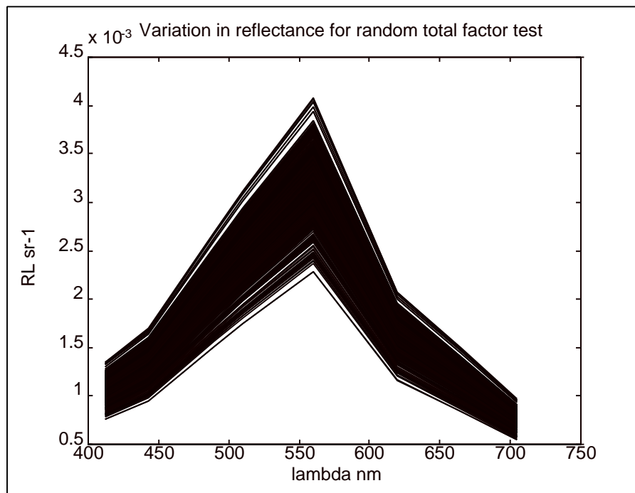
Fig. 14 Variation of reflectance spectra produced by multiplying the whole spectrum with a N(1, 0.01) -distributed random number. Target concentration for chlorophyll is 4 \mu\text{g/l} , NSP 2 \text{ mg/l} and gelbstoff absorption at 440 \text{ nm} of 0.5 \text{ m}^{-1} .
