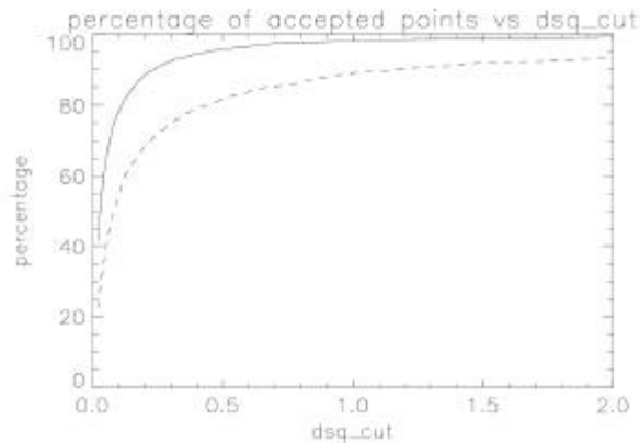
fig. 10 Percentage of points with dsq < dsq\_cut as a function of dsq\_cut is shown for the test samples corresponding to the error model (line) and to 3 times the error model (dashed)
