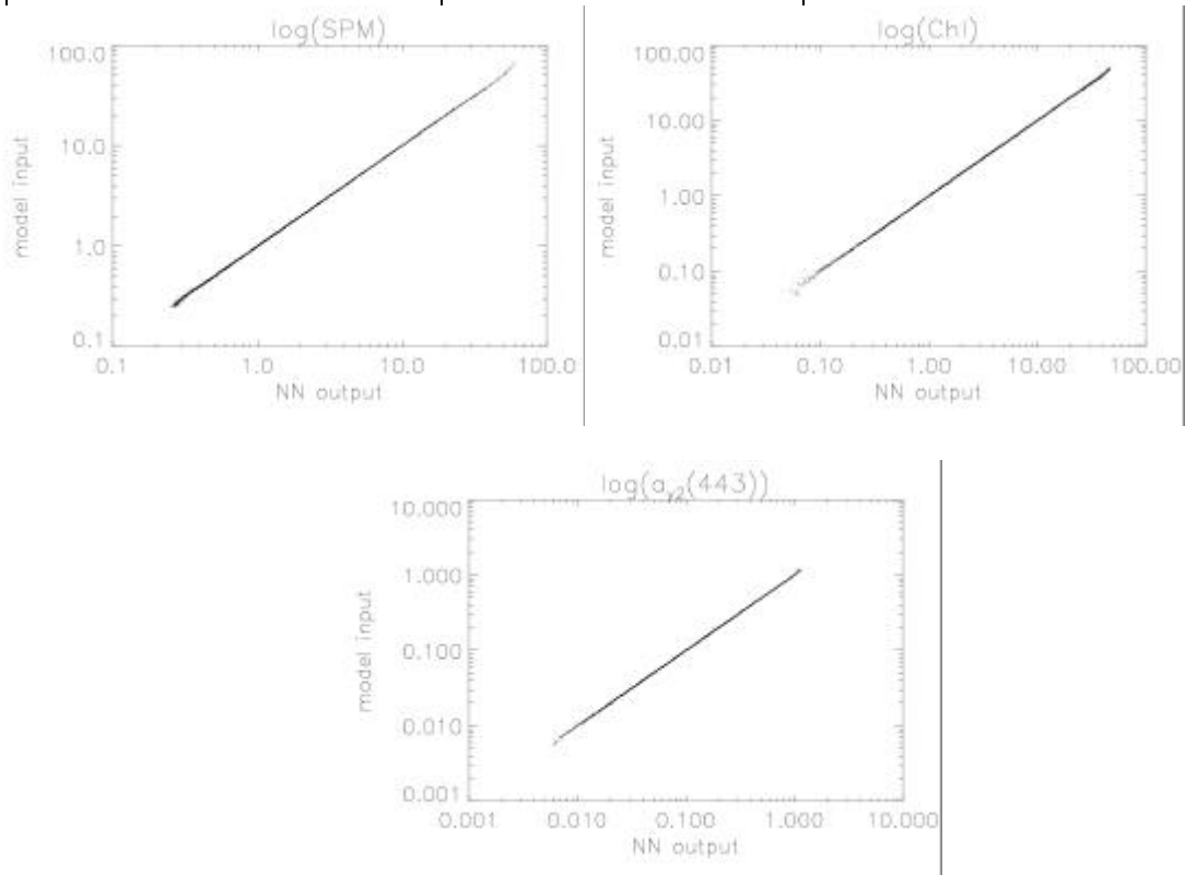
fig. 5 Performance of inverse NN trained with noise-free data
