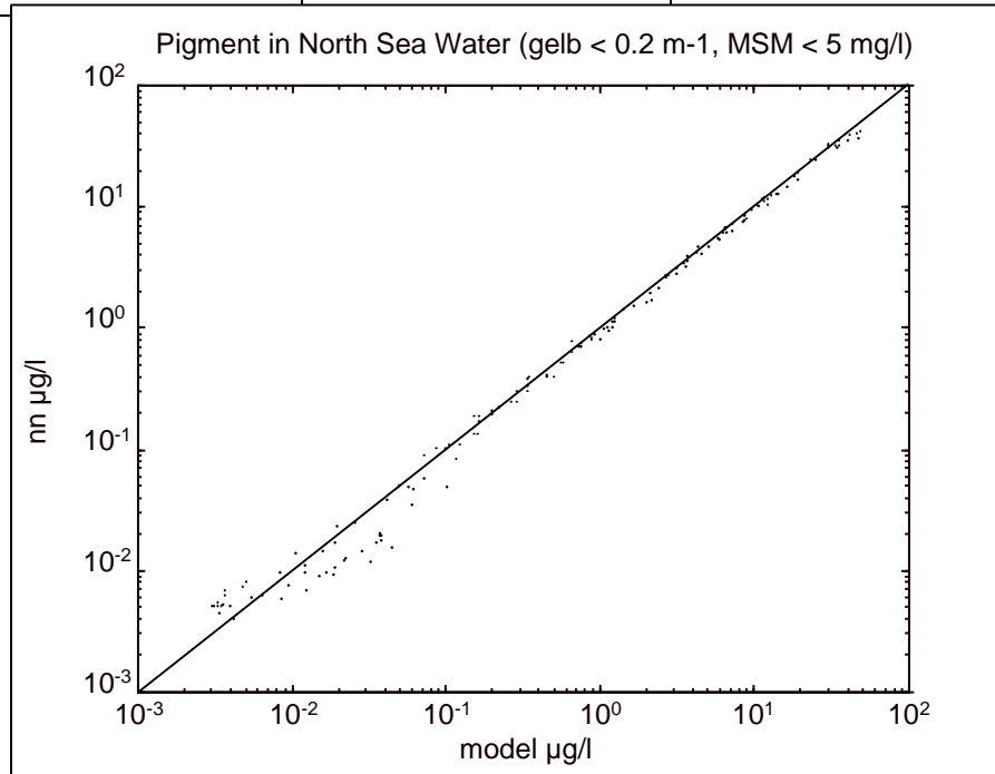
Fig. 12 Input and NN derived concentration of phytoplankton pigment (chlorophyll a) for typical North Sea water
