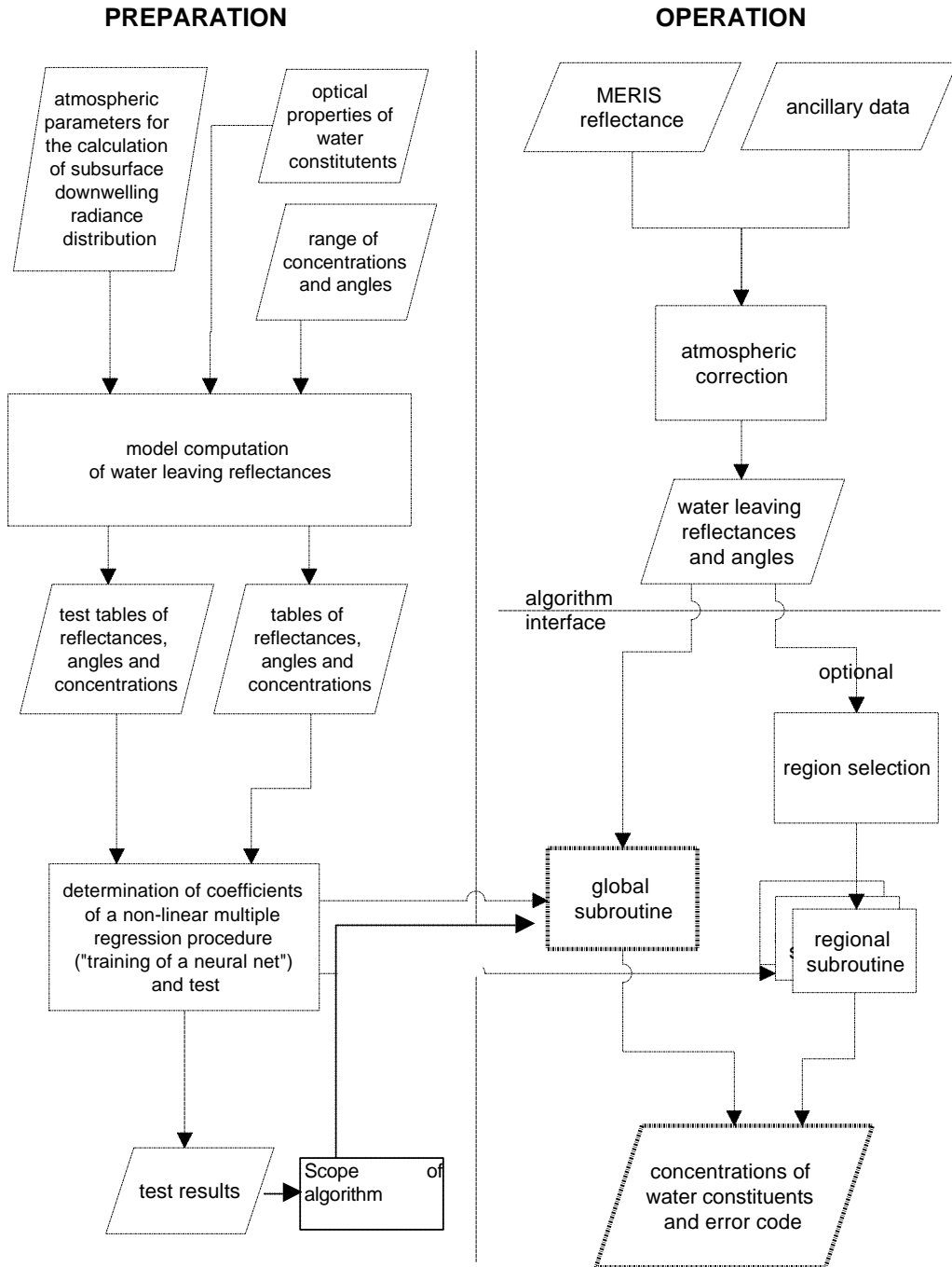
Fig. 1 Scheme of the algorithm based on inverse modelling of radiative transfer and its parametrization with a multiple non-linear regression procedure ("feed forward backpropagation neural network"). The scheme includes the option of different training sets for different coastal regions.
