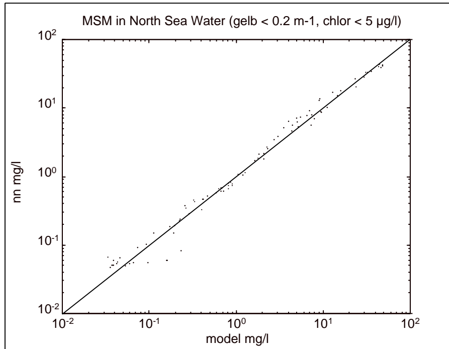
Fig. 13 Input and NN derived concentration of mineralic suspended matter for typical North Sea water
